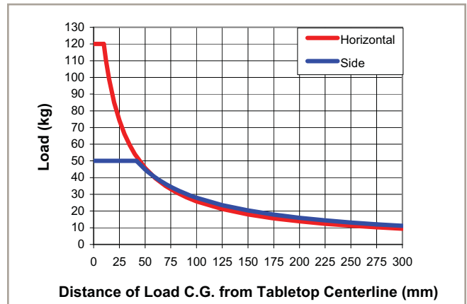
ABL8000-LC Cantilevered Load Capability
