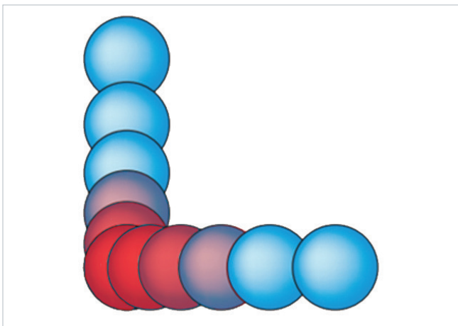
Figure 1. Laser spot placement without PSO. Notice the uneven overlap evident when changing direction which causes inconsistent energy delivery to the workpiece resulting in poor part quality.
