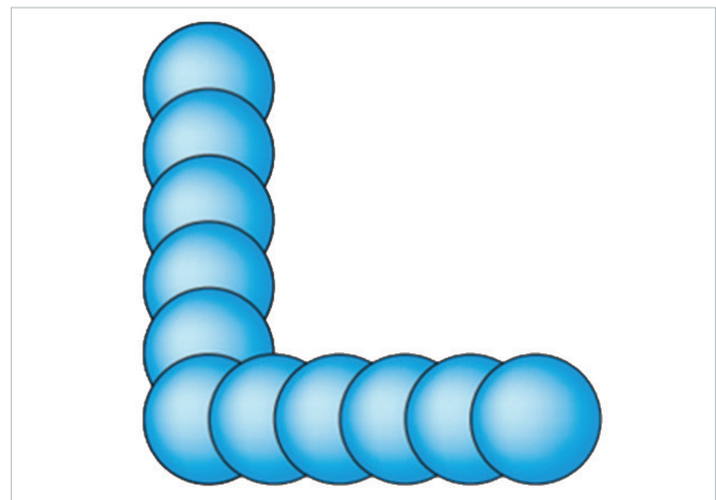
Figure 2. Laser spot placement with PSO. Notice the even overlap, even when changing direction, when Aerotech's PSO is applied. This results in consistent energy delivery and better part quality.
