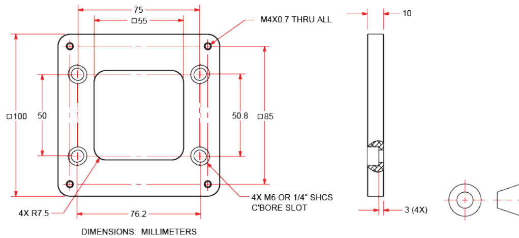
Figure 2-5: QNP2-100XYA-100 Mounting Plate (-MP) Dimensions
