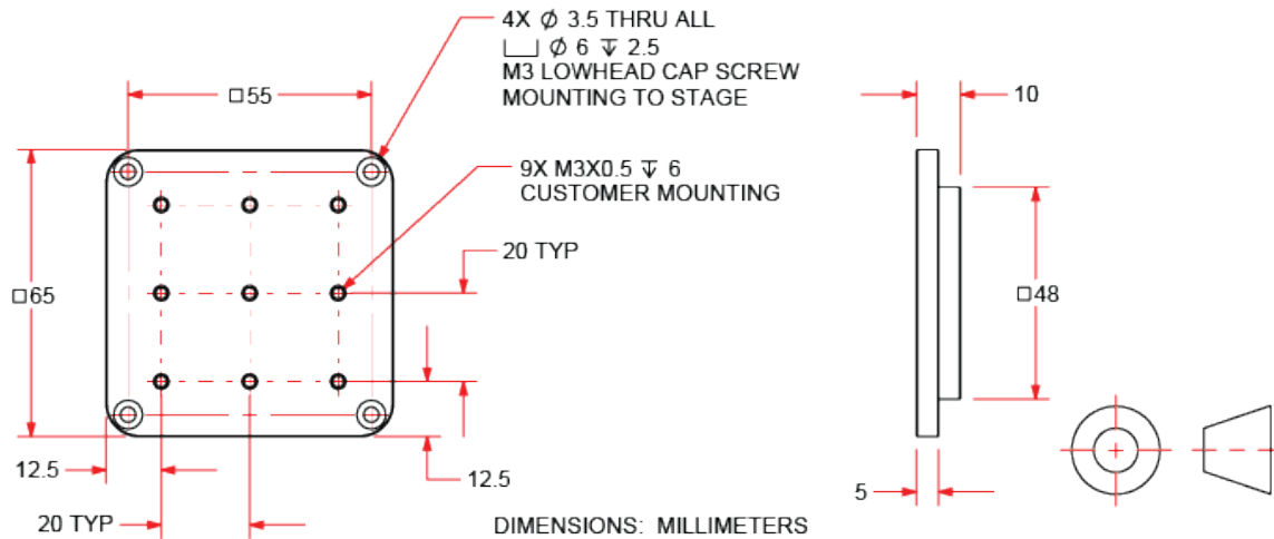
Figure 2-8: QNP2-100XYA-100 Tabletop (-TT1) Dimensions
