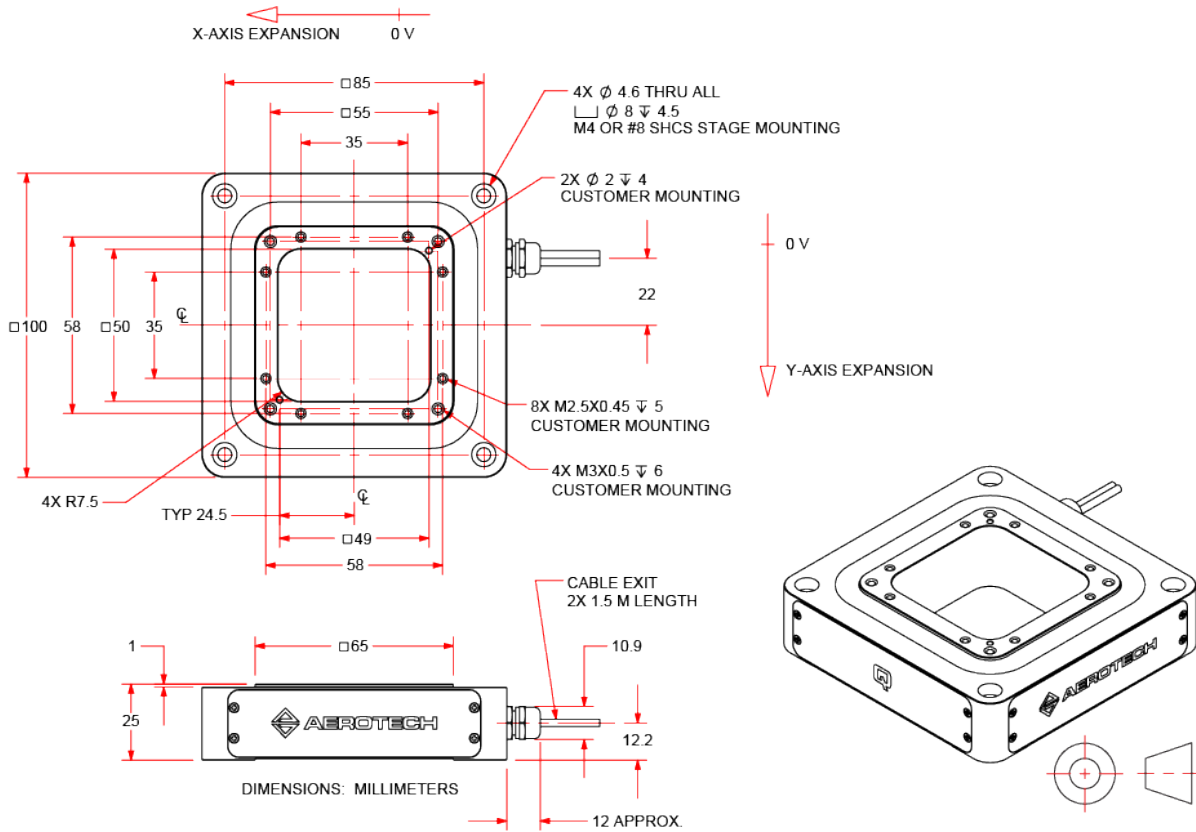
Figure 2-2: QNP2-100XYA-100 Dimensions
