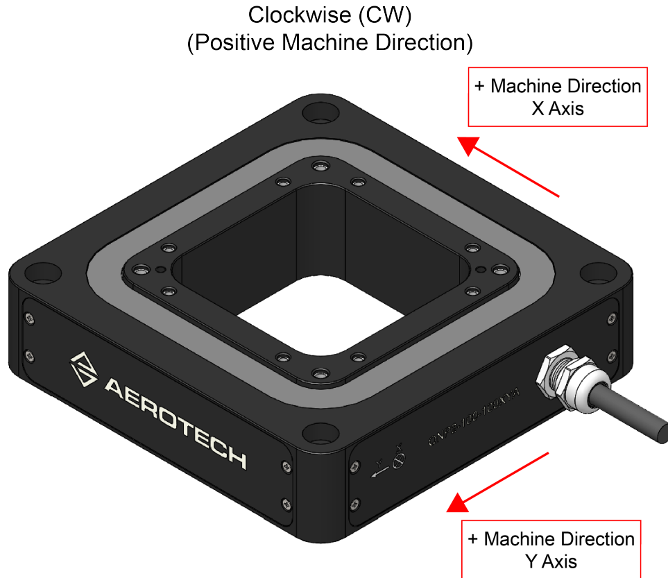
Figure 3-2: Machine Direction
