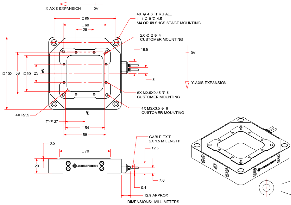
Figure 2-1: QNP2-100XYA-030 Dimensions
