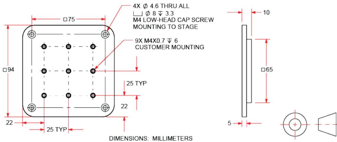
Figure 2-9: QNP2-200XYA-200 Tabletop (-TT1) Dimensions
