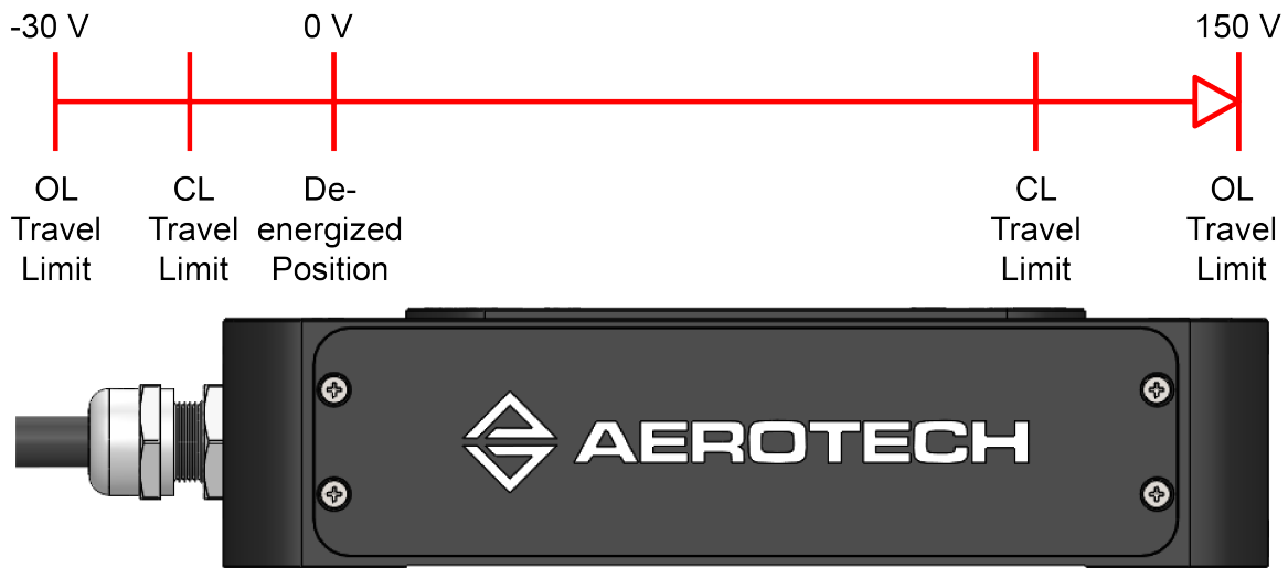
Figure 1-1: Single-Axis Stage Travel and Voltage Relationship
