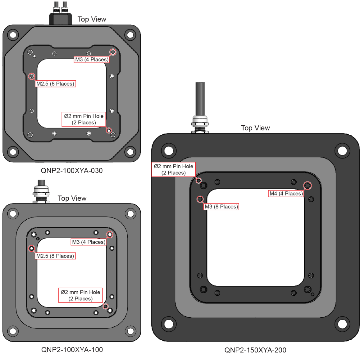
Figure 2-11: Mounting Hole Locations (Tabletop)
