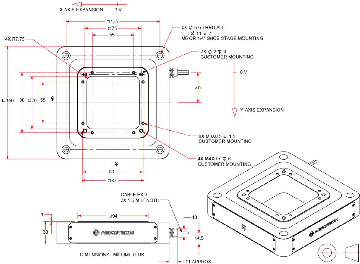
Figure 2-3: QNP2-150XYA-200 Dimensions
