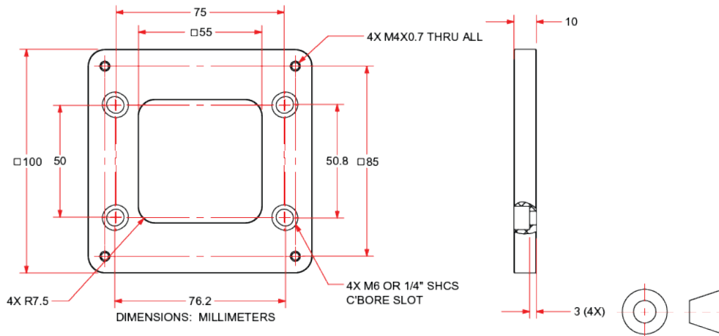
Figure 2-4: QNP2-100XYA-030 Mounting Plate (-MP) Dimensions
