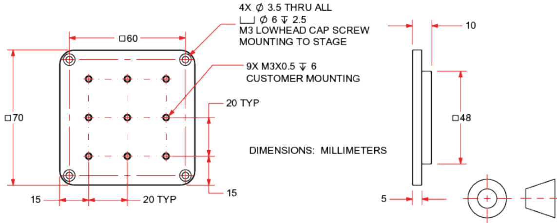
Figure 2-7: QNP2-100XYA-030 Tabletop (-TT1) Dimensions
