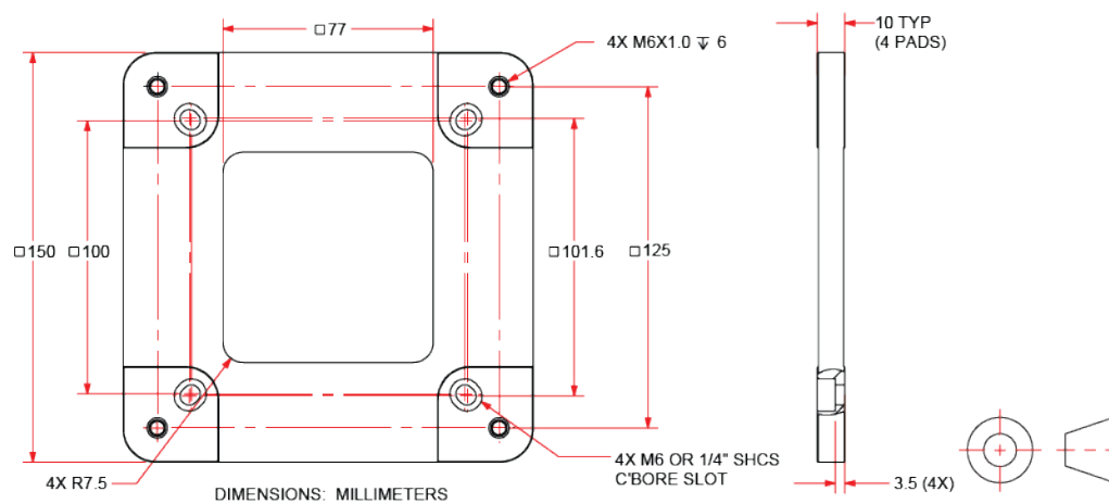
Figure 2-6: QNP2-150XYA-200 Mounting Plate (-MP) Dimensions
