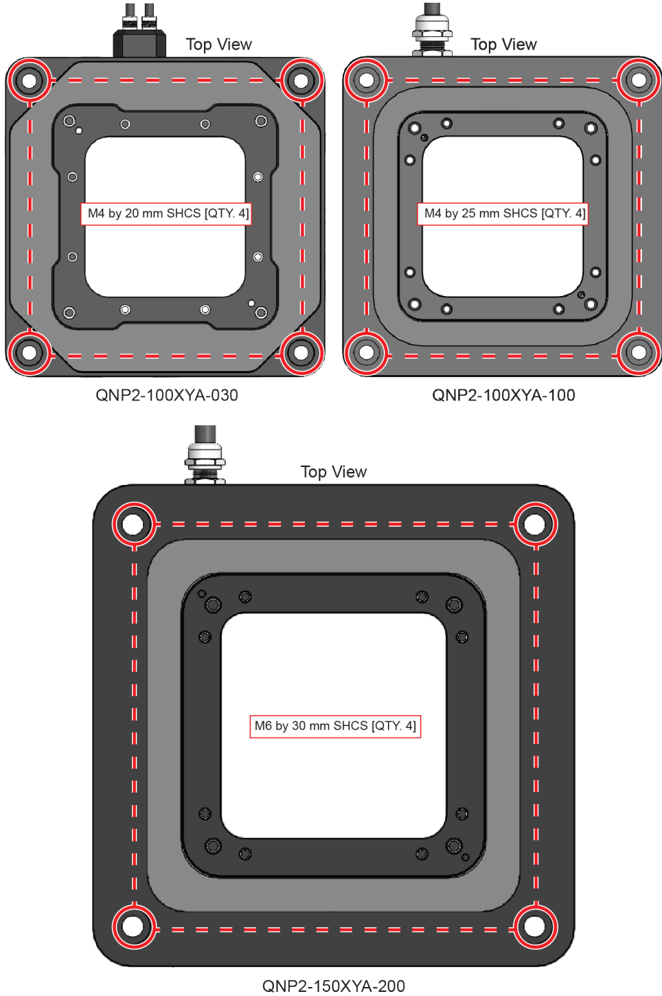
Figure 2-10: Mounting Hole Locations
