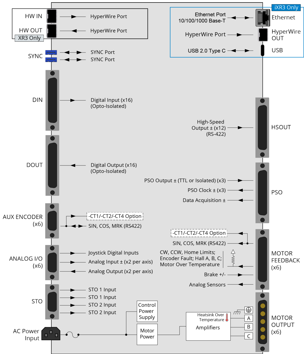
Figure 1-1: Functional Diagram
