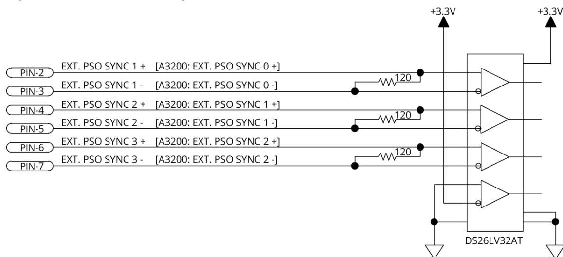
Figure 2-29: PSO Clock Inputs Schematic
