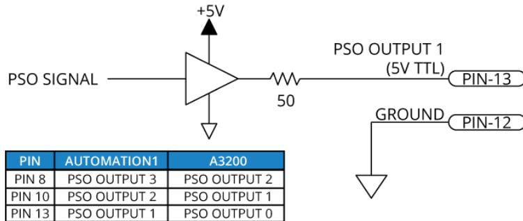
Figure 2-28: PSO TTL Outputs Schematic
