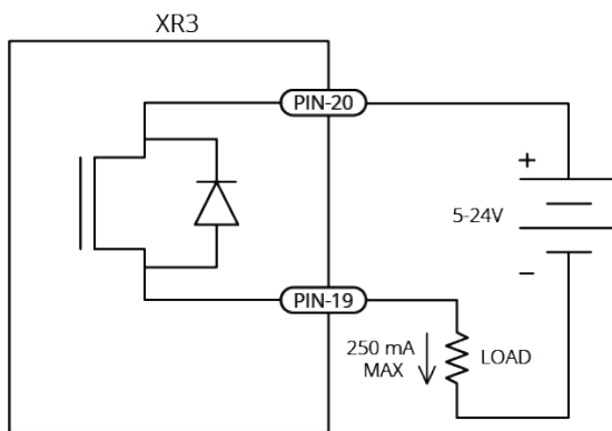
Figure 2-26: PSO Output Sources Current
