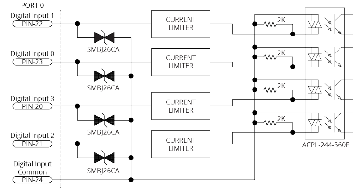
Figure 2-35: Digital Input Schematic
