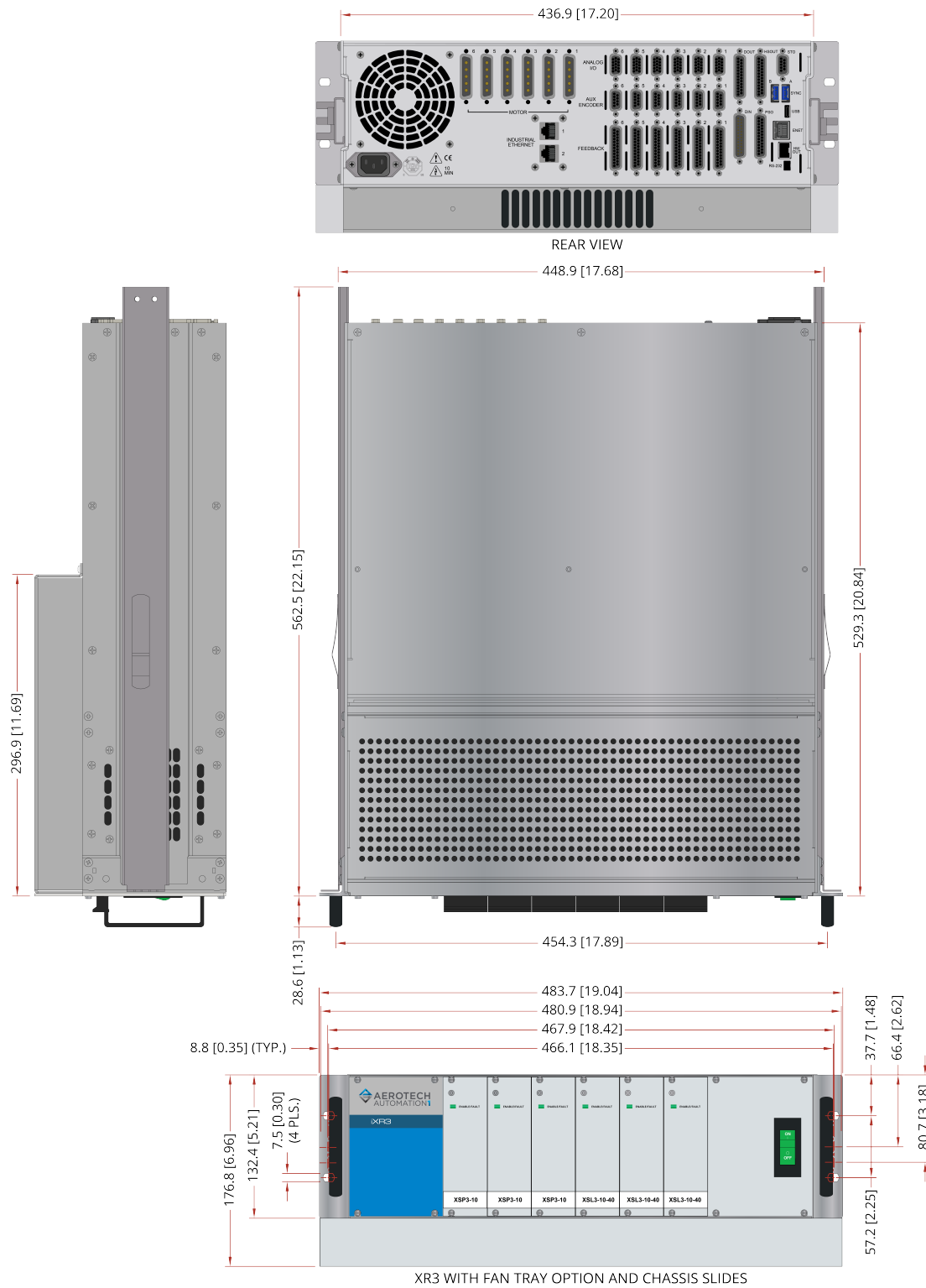
Figure 1-3: Dimensions with Chassis Slides
