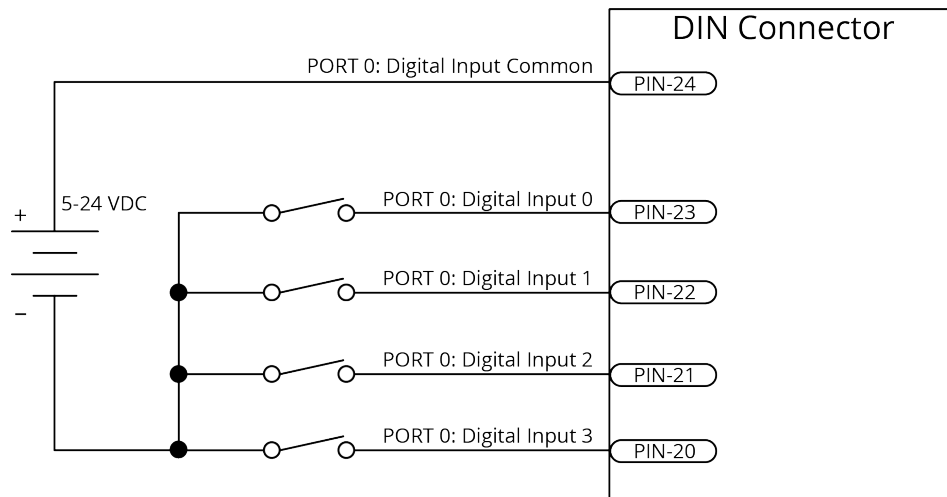
Figure 2-37: Digital Inputs Connected to Current Sinking (NPN) Devices
