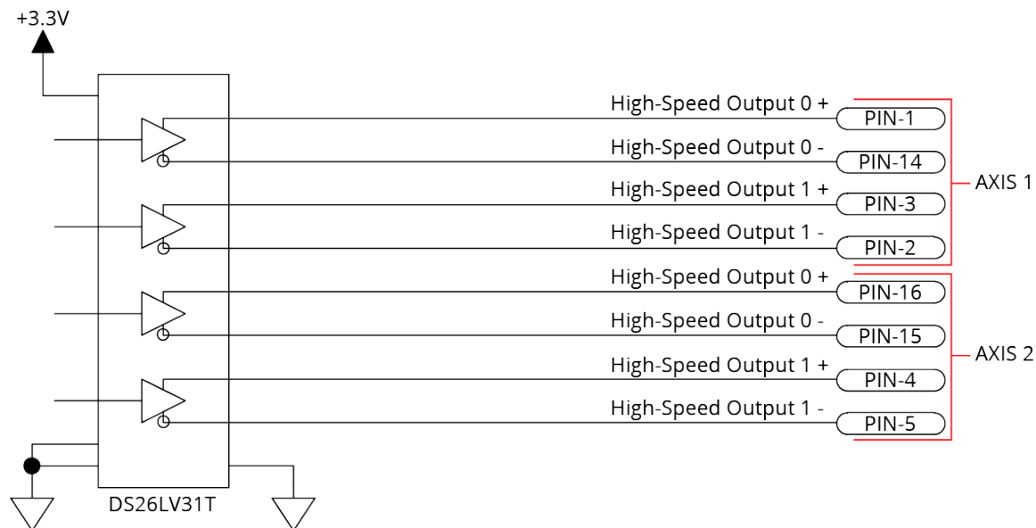
Figure 2-31: Diagram Showing Axis 1 and Axis 2 High-Speed Outputs
