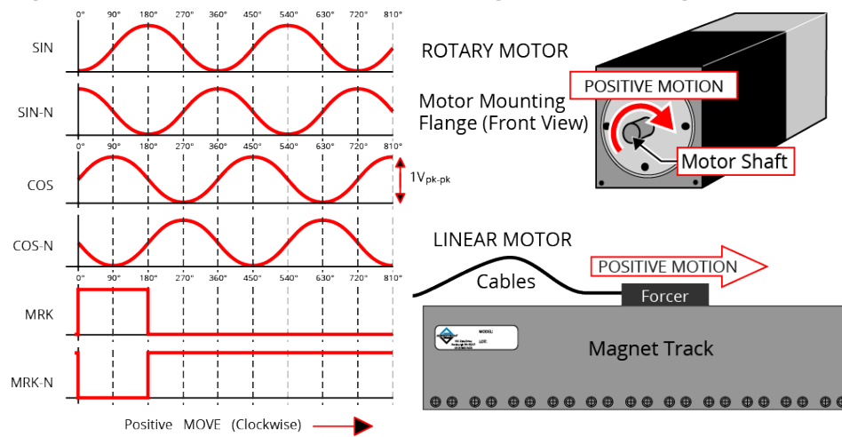
Figure 2-40: Sine Wave Encoder Phasing Reference Diagram
