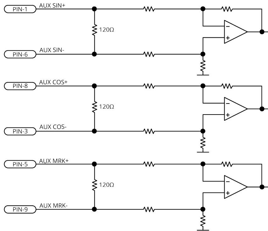
Figure 2-41: Sine Wave Encoder Schematic (Aux Encoder Connector)
