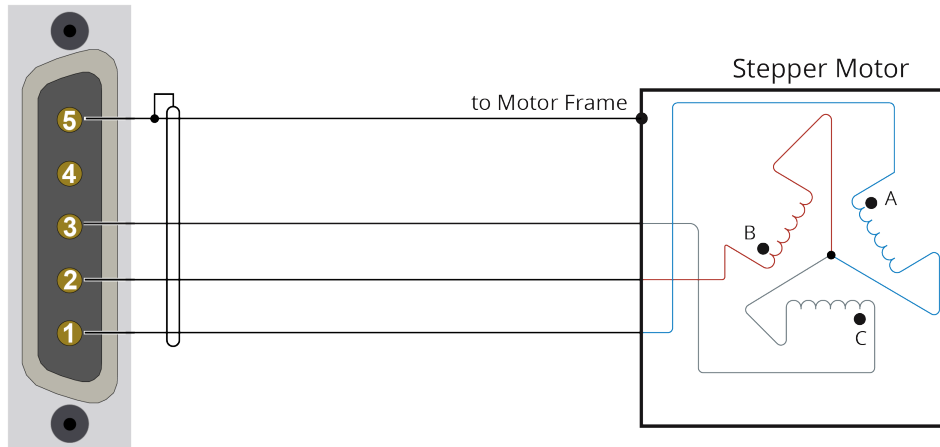
Figure 2-11: Three Phase Stepper Motor Configuration
