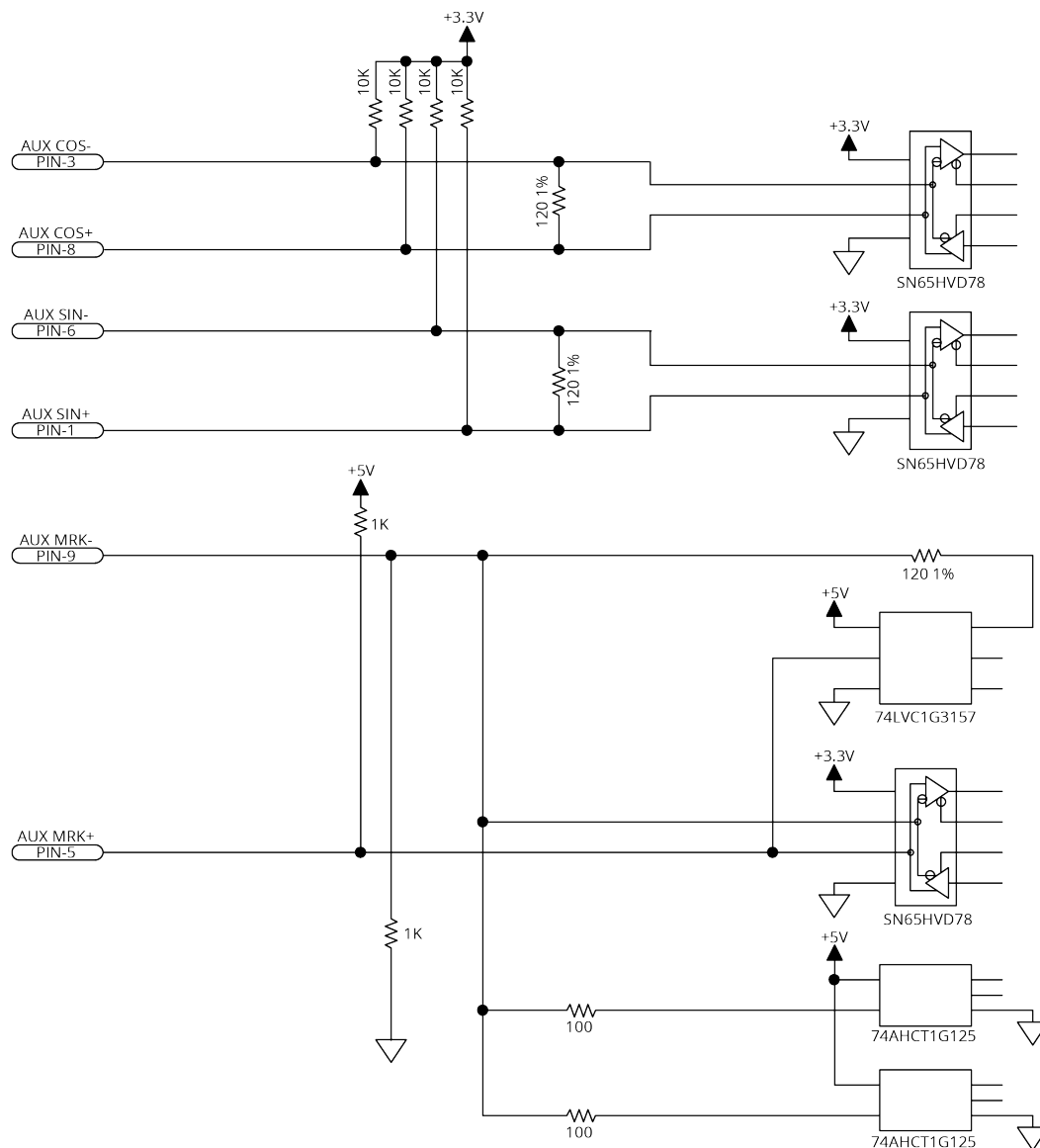
Figure 2-38: Square Wave Encoder Interface (Aux Encoder Connector)
