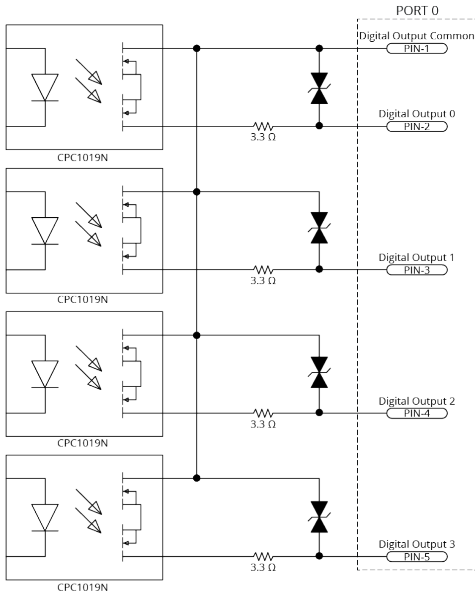
Figure 2-32: Digital Output Schematic
