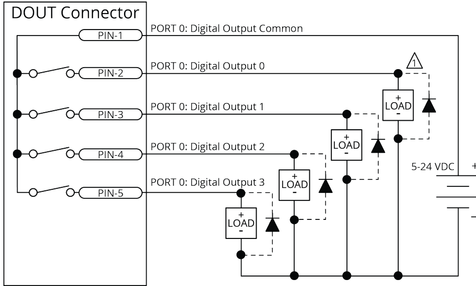
Figure 2-33: Digital Outputs Connected in Current Sourcing Mode
