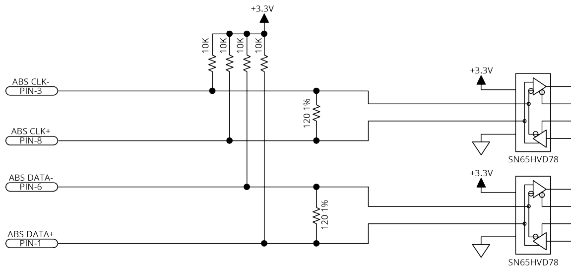
Figure 2-39: Absolute Encoder Schematic (Aux Encoder Connector)
