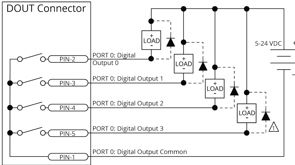
Figure 2-34: Outputs Connected in Current Sinking Mode
