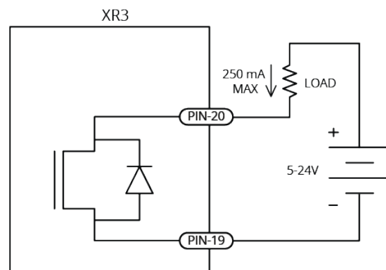
Figure 2-27: PSO Output Sinks Current
