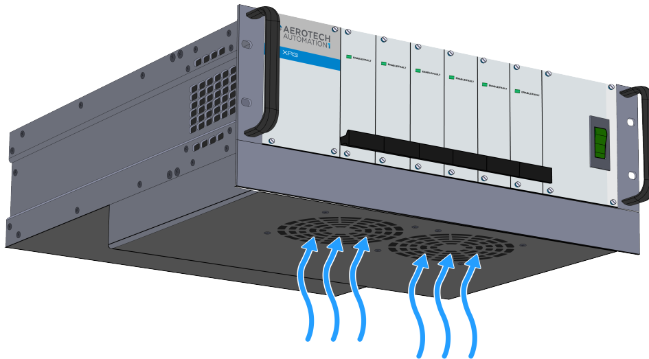
Figure 2-51: -C2 1U Fan Location and Air Flow
