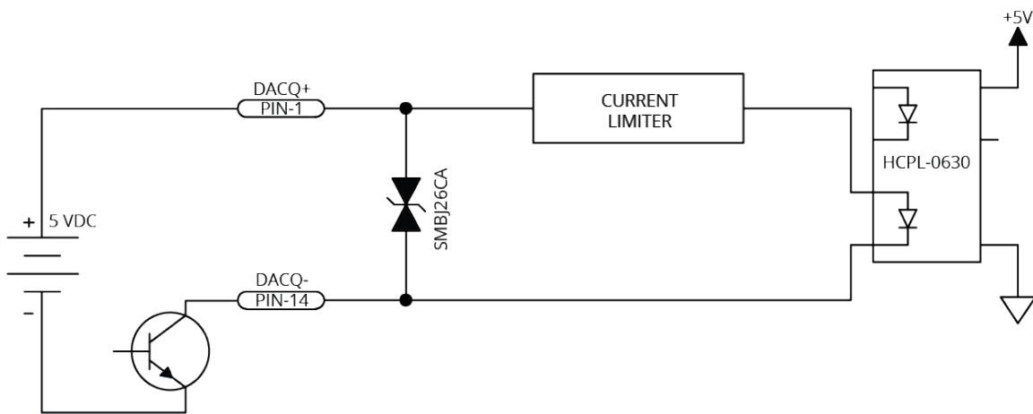
Figure 2-30: Data Acquisition Input Schematic
