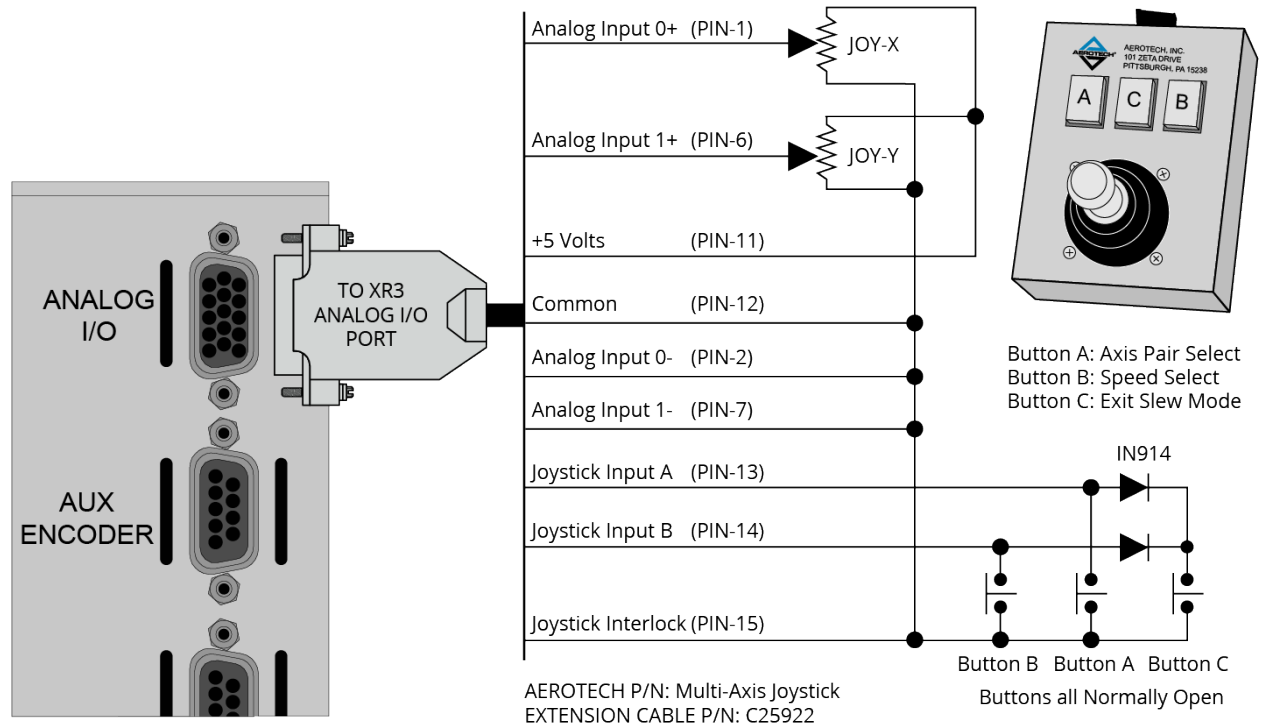
Figure 2-45: Joystick Cable Wiring Schematic
