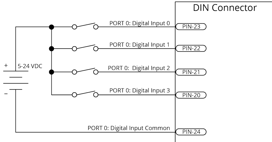
Figure 2-36: Digital Inputs Connected to Current Sourcing (PNP) Devices
