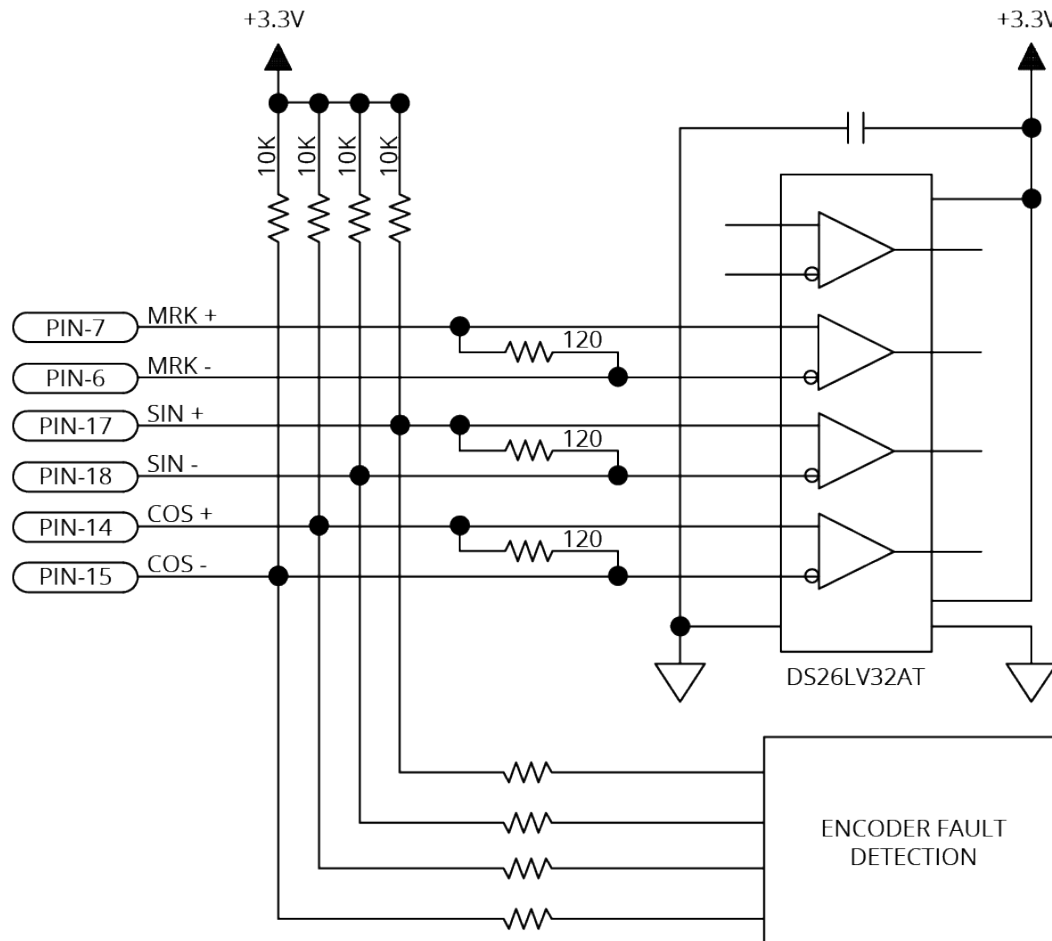
Figure 2-13: Square Wave Encoder Schematic (Feedback Connector)
