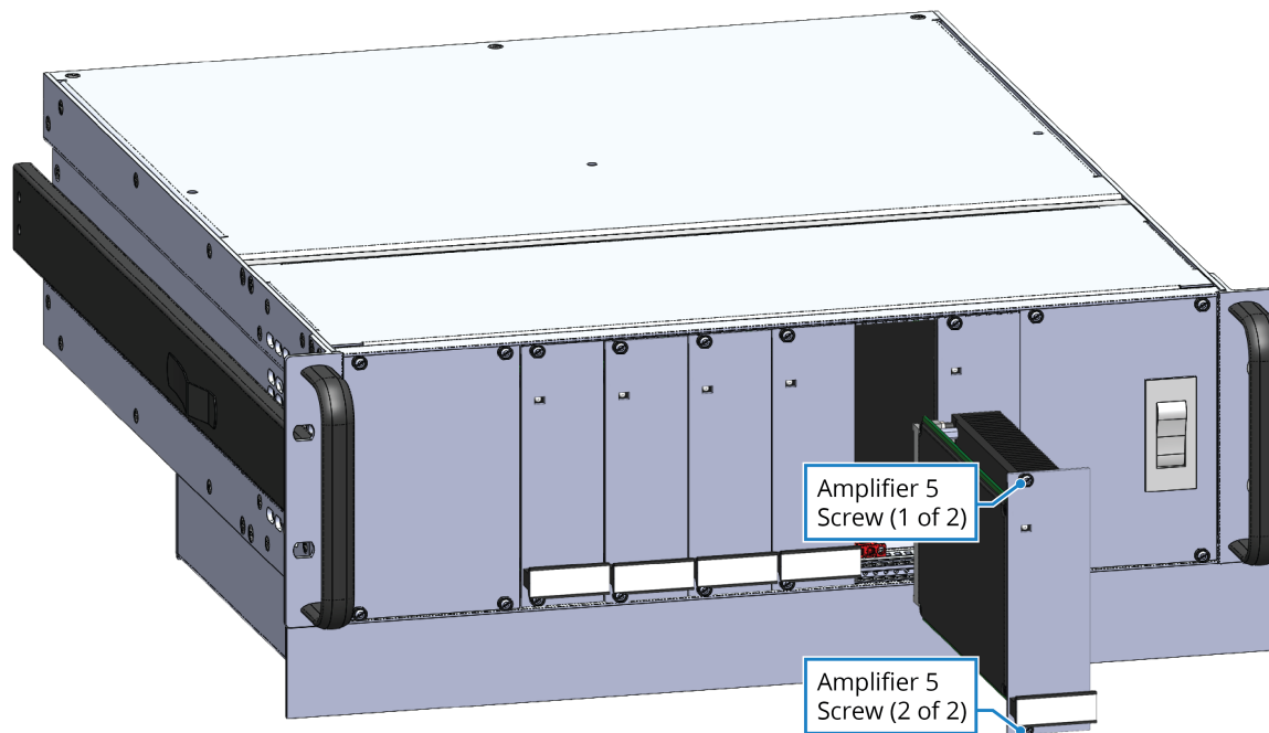
Figure 3-2: Amplifier Removal
