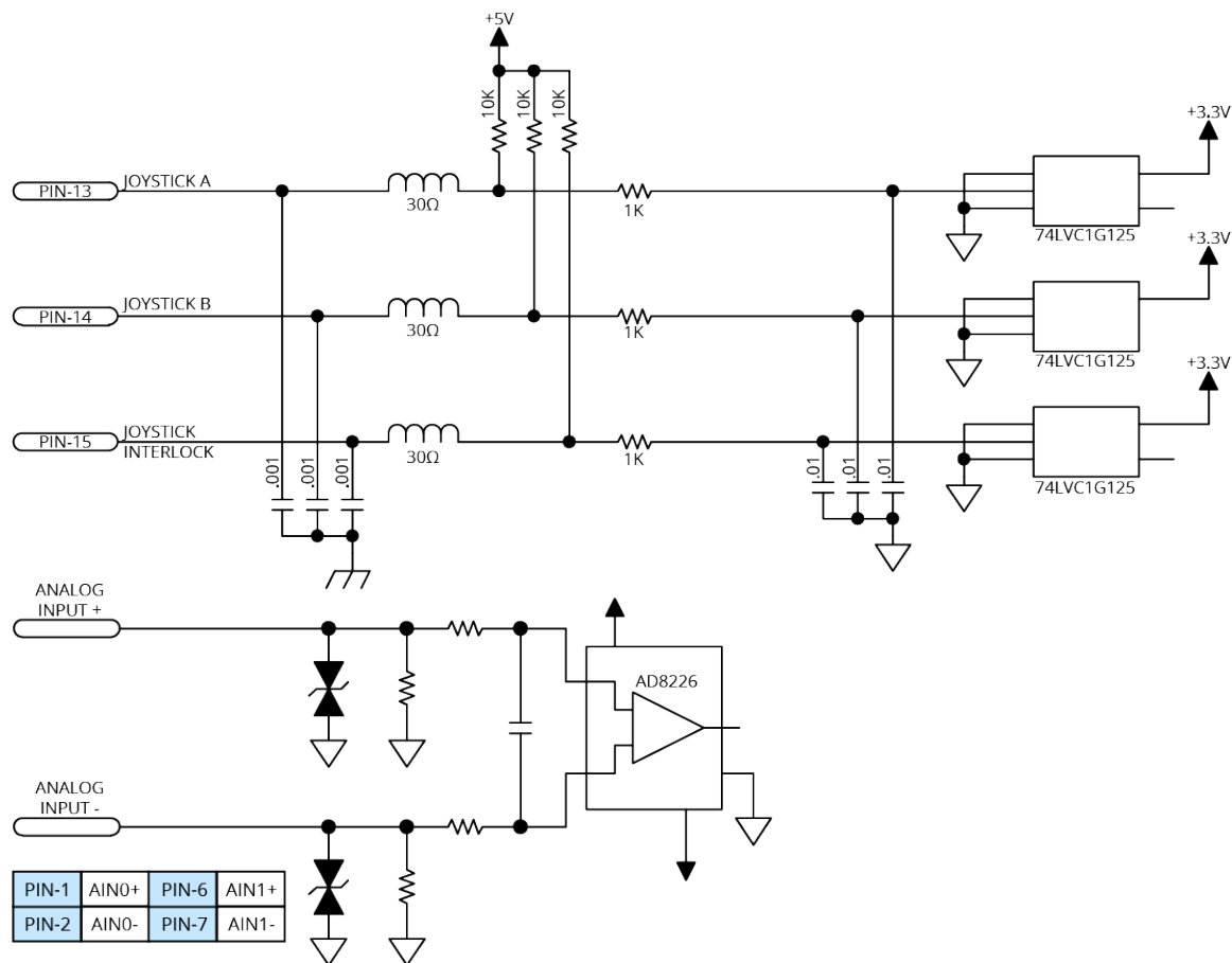
Figure 2-44: Joystick Interface Inputs Schematic
