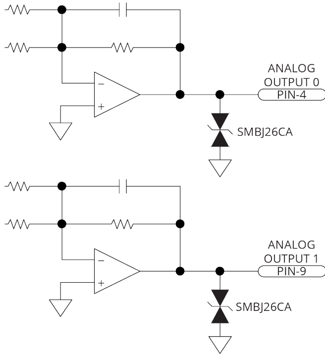
Figure 2-42: Analog Outputs Schematic
