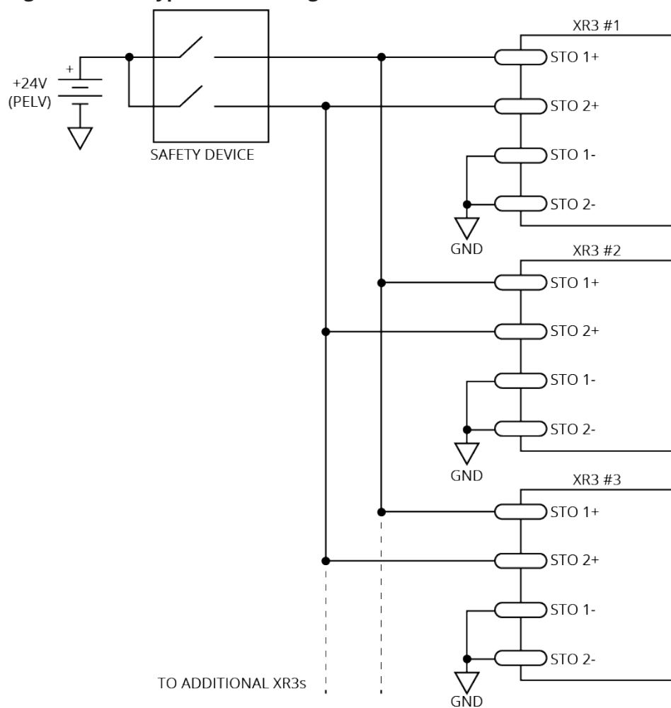
Figure 2-46: Typical STO Configuration
